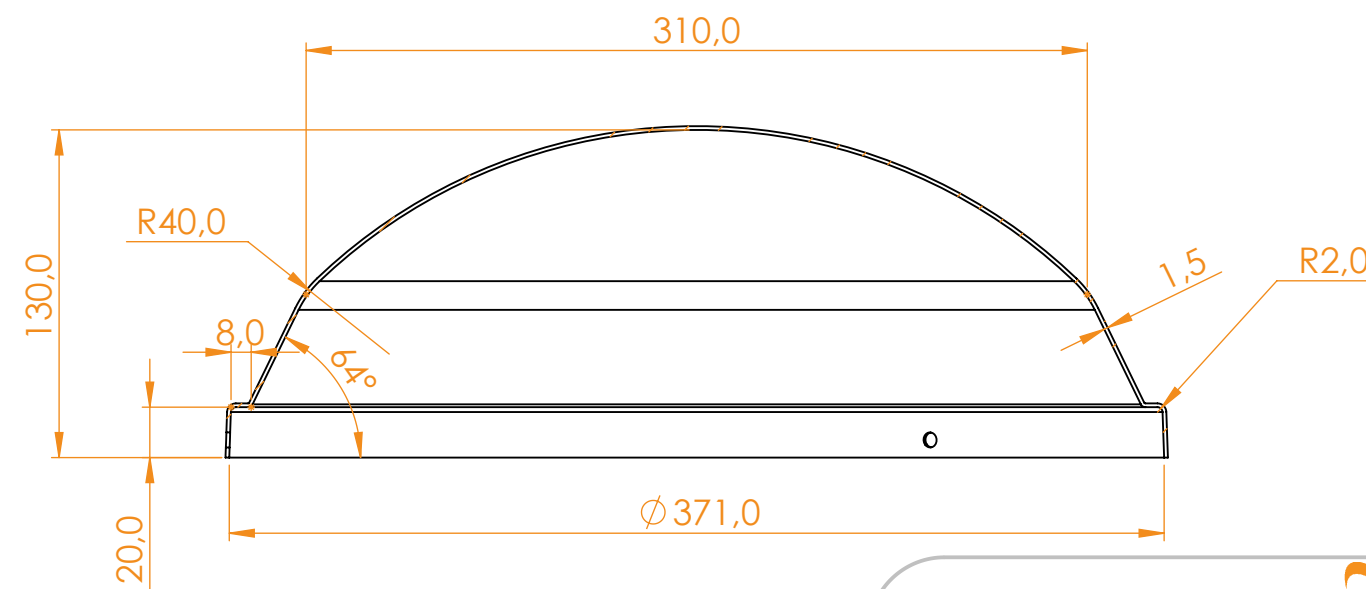
SECTION C-C
