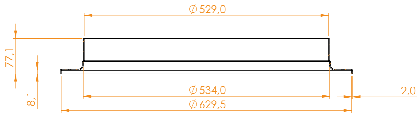
SECTION C-C
